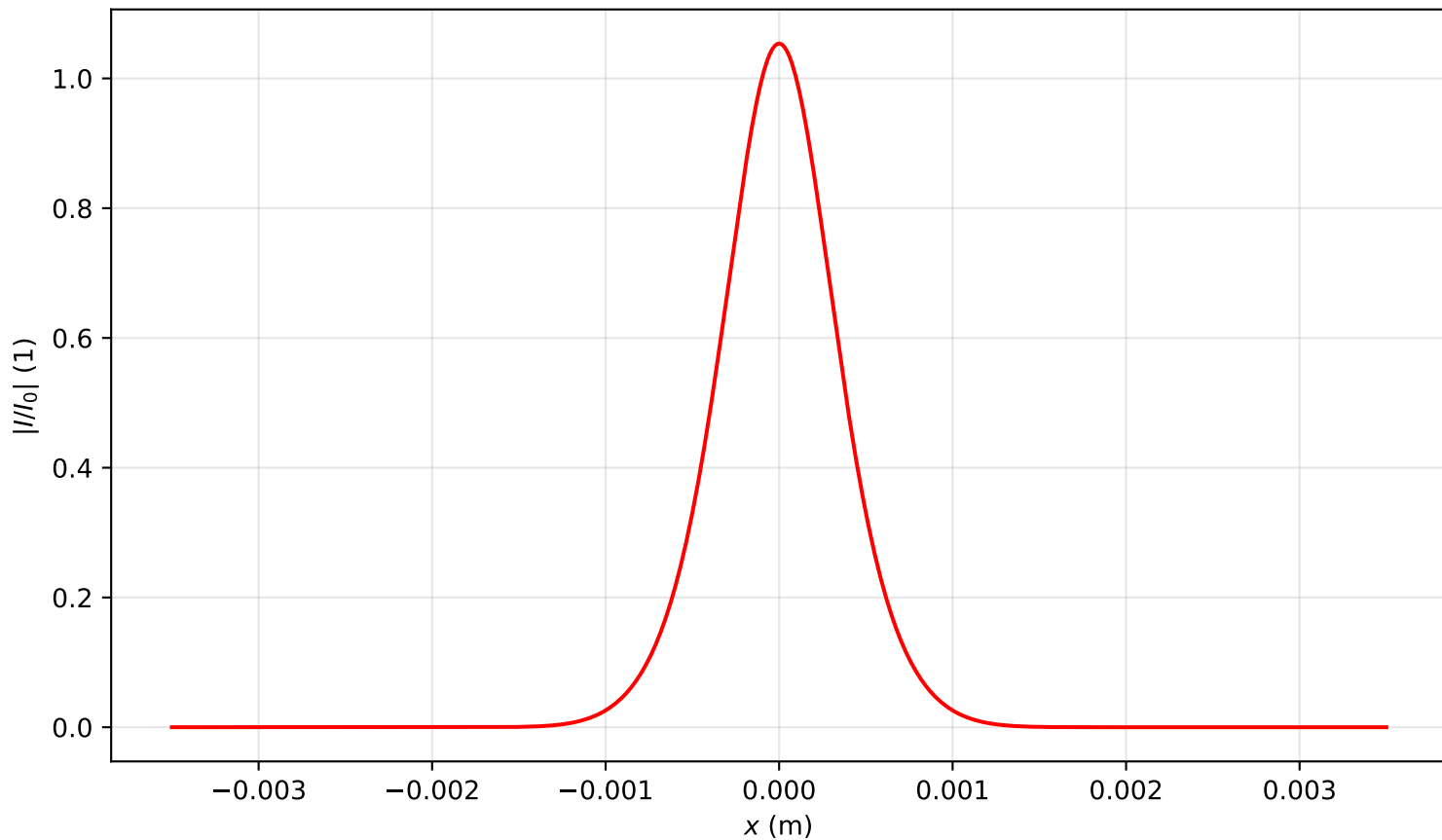
Intensity profile I(x, y = 0, z = 0.955)/I_0 , P_{in}=0.5P_{cr} , artificial time
